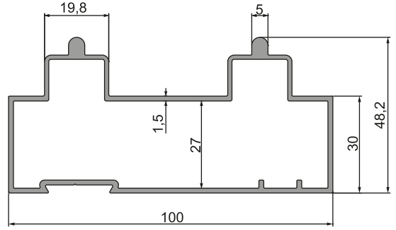
14-002 (1,367 kg/m)
