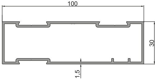
12-010 (1,134 kg/m)
