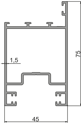
14-003 (1,157 kg/m)
