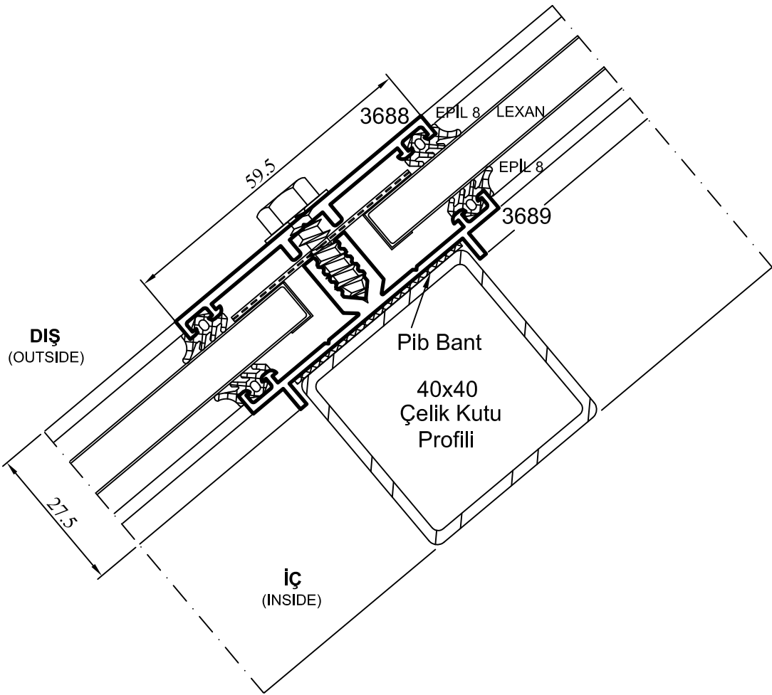
Detay Detail 2
