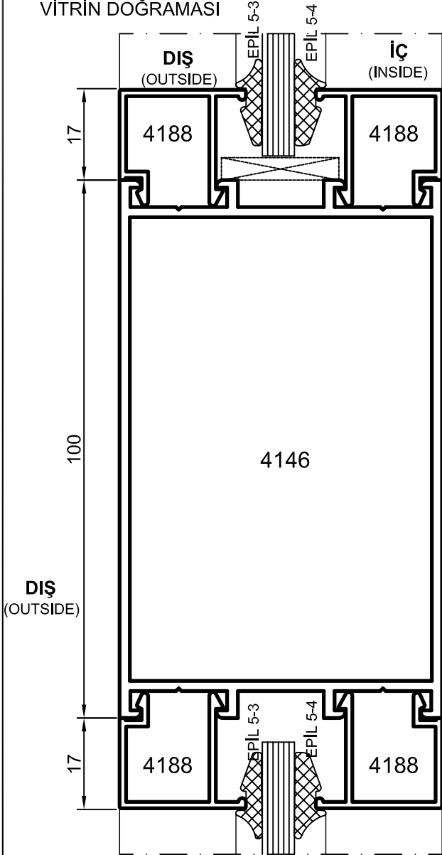
Detay Detail 4
