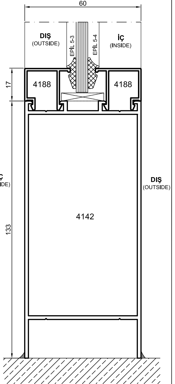
Detay Detail 5
