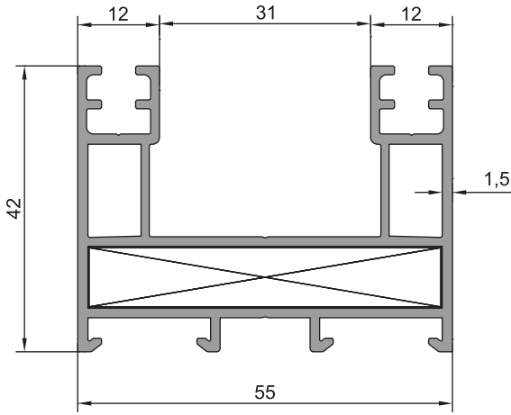
KASA PROFİLİ 26-001 (1,102 kg/m) Jx: 16,72 cm 4 / Jy: 6,27 cm 4
