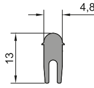
RAY PROFİLİ 26-016 (0,125kg/m)
