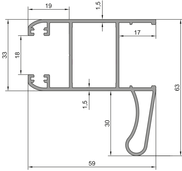
TAKVİYELİ KANAT PROFİLİ 26-005 (1,053kg/m) Jx: 18,09 cm 4 / Jy: 7,69 cm 4
