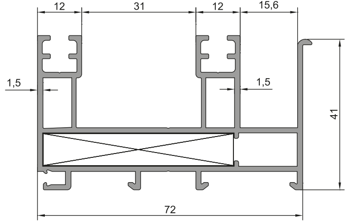
2'Lİ PERVAZLI KASA PROFİLİ 26-002 (1,350 kg/m) Jx: 30,08 cm 4 / Jy: 7,52 cm 4
