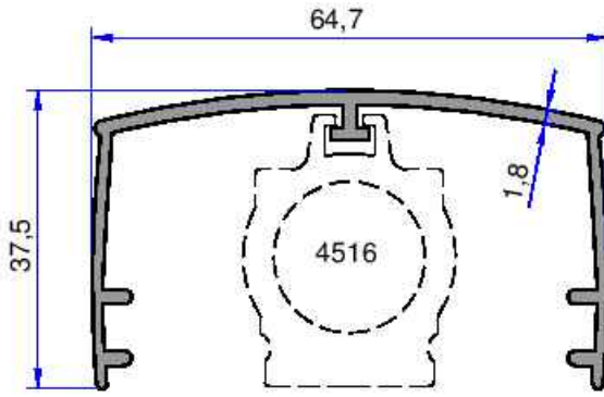
4523 0.660 kg/m
