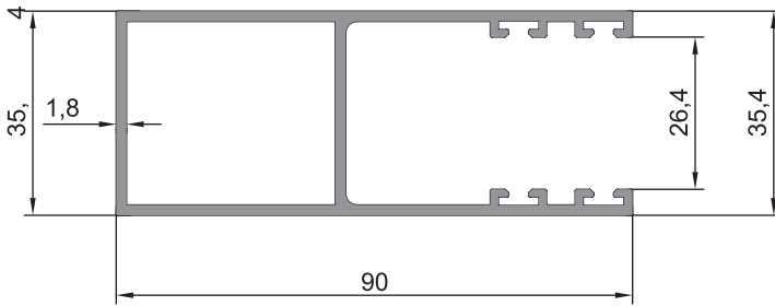
09-013 (1,313 kg/m)
