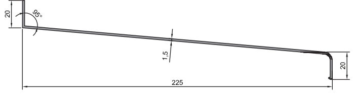
07 - 011 (1,126 kg/m)
